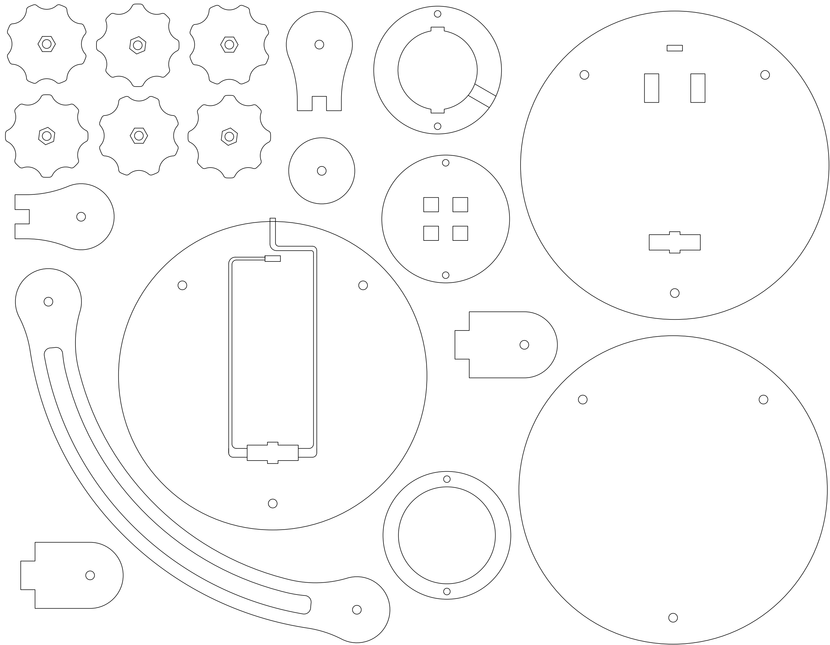
Desk Lamp - ZenziWerken - 6.5 mm Beech Plywood / 4 mm High Density Fiberboard
