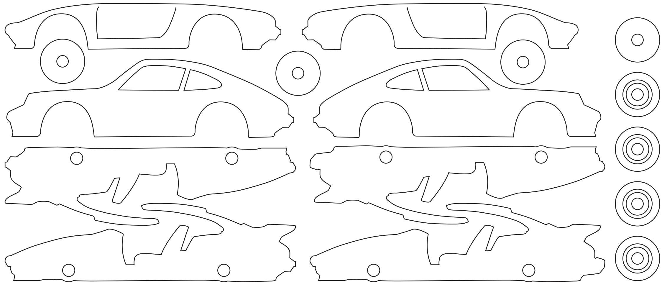
Porsche 911 simplified - ZenziWerken - 6.5 mm Plywood
